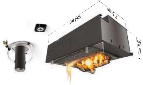
L-FIRE BURNER
